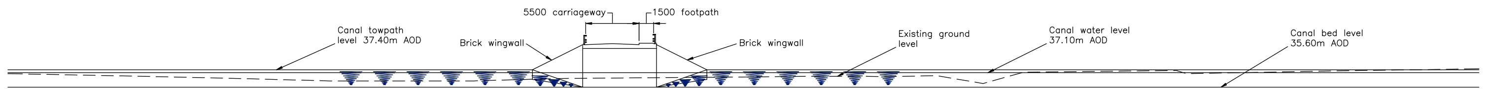
Long section of canal through Rugby Club access road
